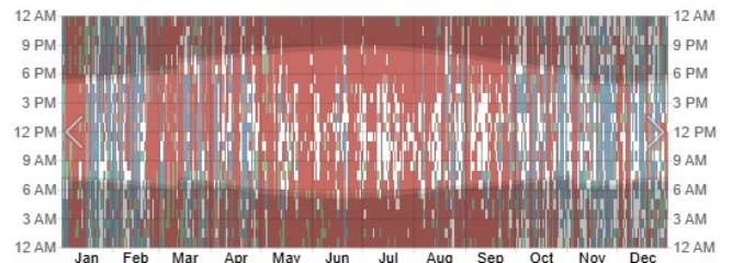
Temperature history in 2023 in Roseville
