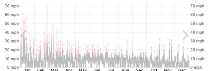
Wind Speed in 2023 in Roseville
