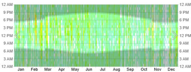
Wind Speed in 2024 in Roseville
